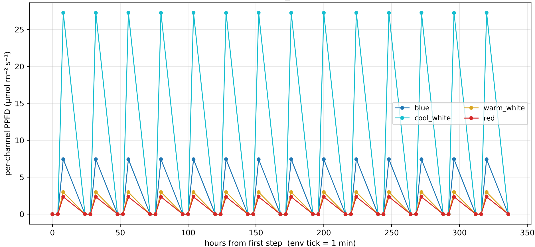
Z3 masked E21-pinned exploit — actions emitted via main_real path (14 sim-days at 1-min env steps, 20160 total)
