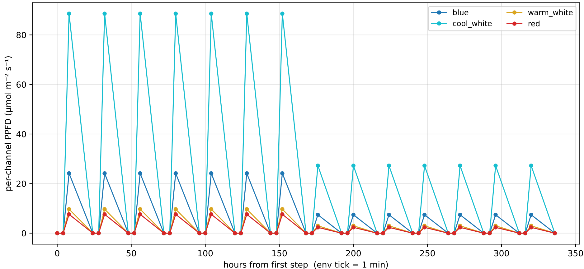
Z4 differential explore (adaptive) — actions emitted via main_real path (14 sim-days at 1-min env steps, 20160 tota
