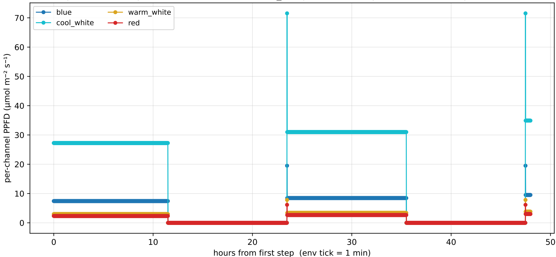
Z1 power-law ramp — actions emitted via main_real path (2 sim-days at 1-min env steps, 2880 total)
