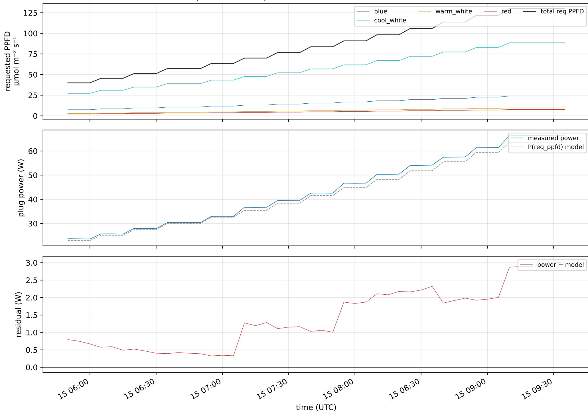
Z1 power-law ramp — actions emitted on the real chamber
