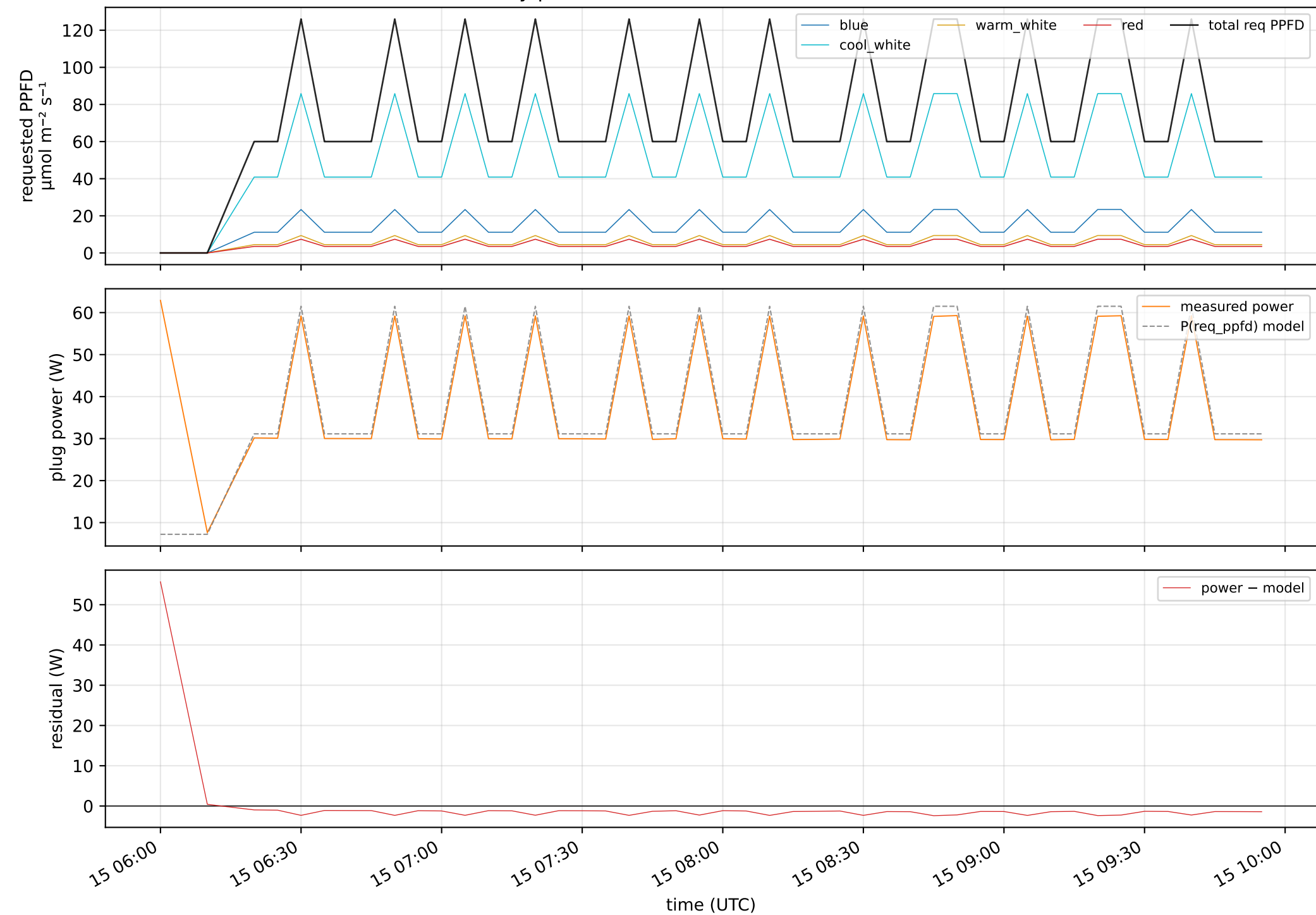
Z2 within-day parabola — actions emitted on the real chamber
