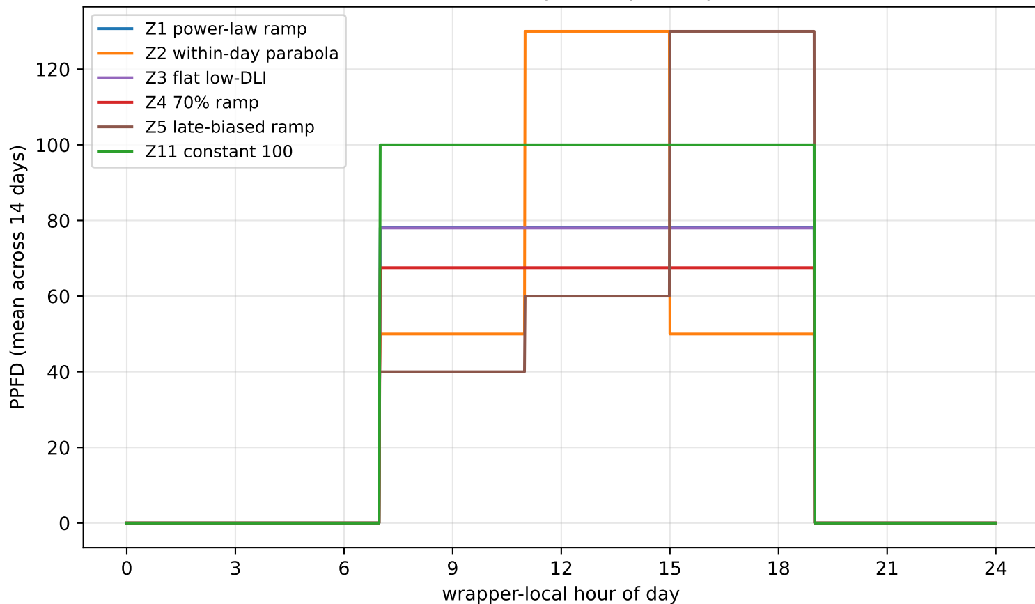
E18/P1 — mean daily PPFD profile per zone
