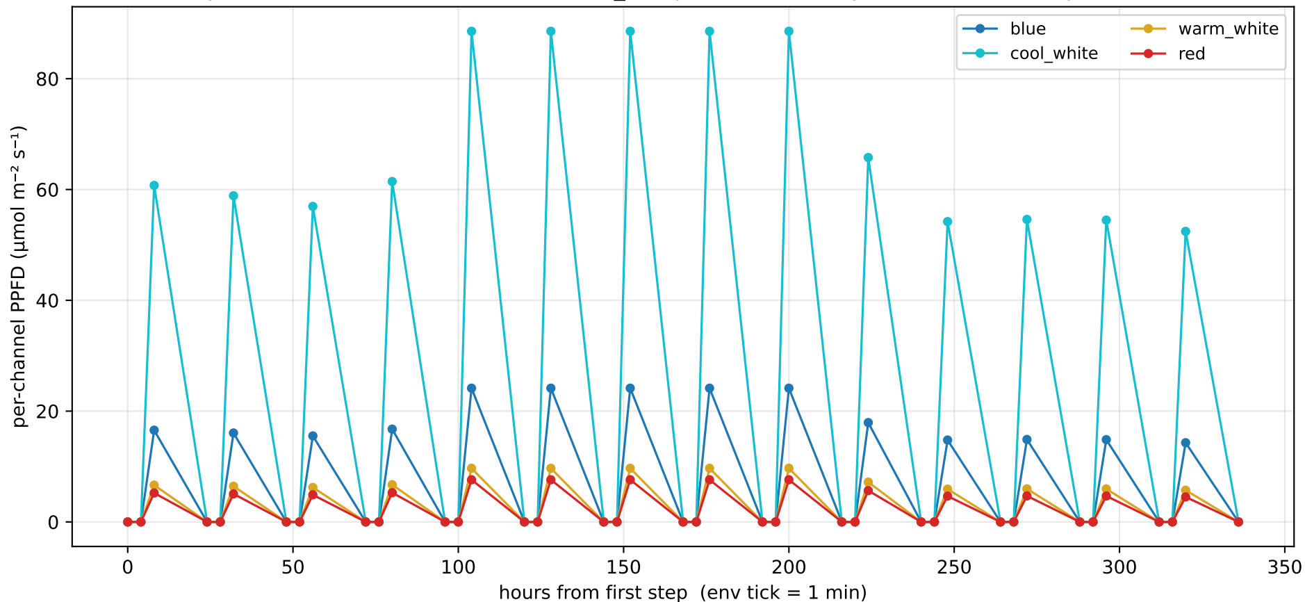
Z1 analytic eval — actions emitted via main_real path (14 sim-days at 1-min env steps, 20160 total)
