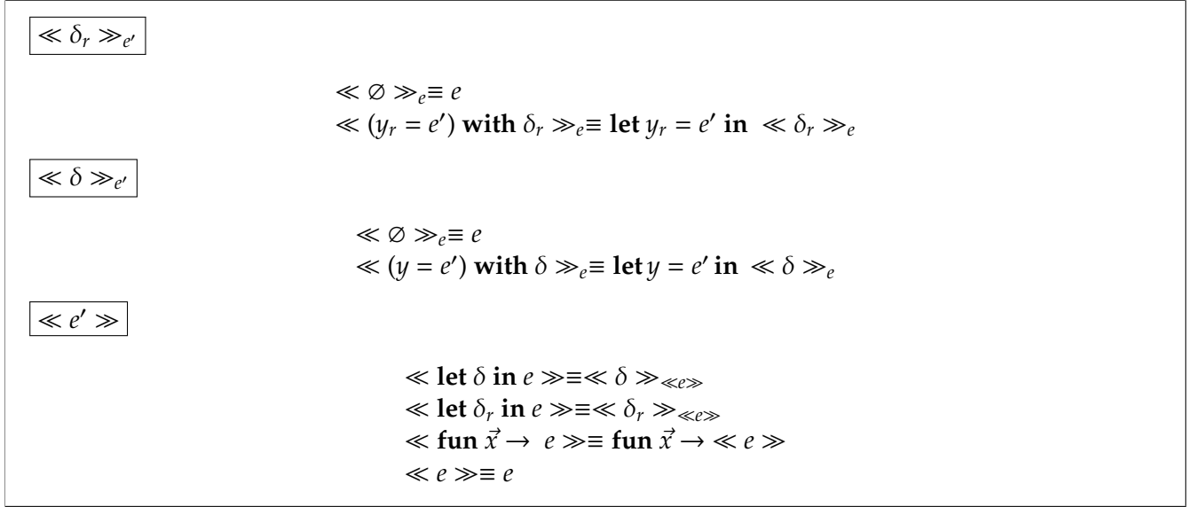
FIGURE 5.5: Function Converting Simultaneous Declarations to Nested Declarations
