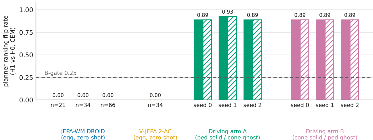
(b) planner flip rate per cell (B-gate tier 2)
