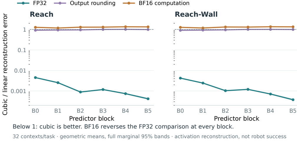
Figure 4: The local reconstruction comparison depends on computation, not only output rounding. Same weights, inputs, action perturbations and coefficients; 32 contexts per task, all six blocks. Curves show geometric mean cubic/linear activation-MSE ratios with full marginal 95% bands. The prespecified paired arithmetic contrasts use six-layer correction. These are reconstruction errors, not forecast or robot-success gains.
