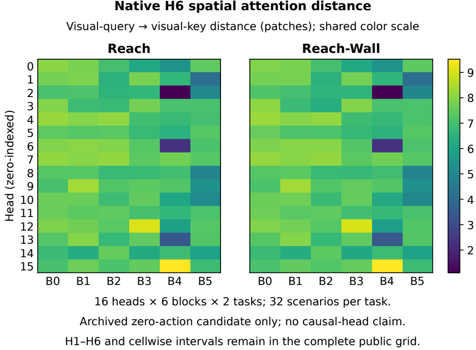
Figure 6: Native H6 attention distance, all six blocks and sixteen heads. Each cell averages 32 development contexts per task with the same archived zero-action candidate. Colors are shared across tasks. The complete H1–H6 grid is retained in the accompanying data. Attention distance is not causal importance or evidence of a planning-emergence zone.
