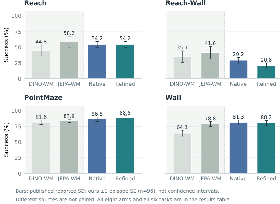
Figure 5: Protected behavior and published benchmarks are distinct evidence. The fixed refined arm and its concurrent native reference use 96 fresh scenarios per task. Shaded DINO-WM/JEPA-WM recipe values are external context. Published error bars are reported late-epoch SD; local bars are one Bernoulli episode SE, not confidence intervals or training-seed variation. No best arm is selected by task. All eight arms and historical rates remain in Appendix C.
