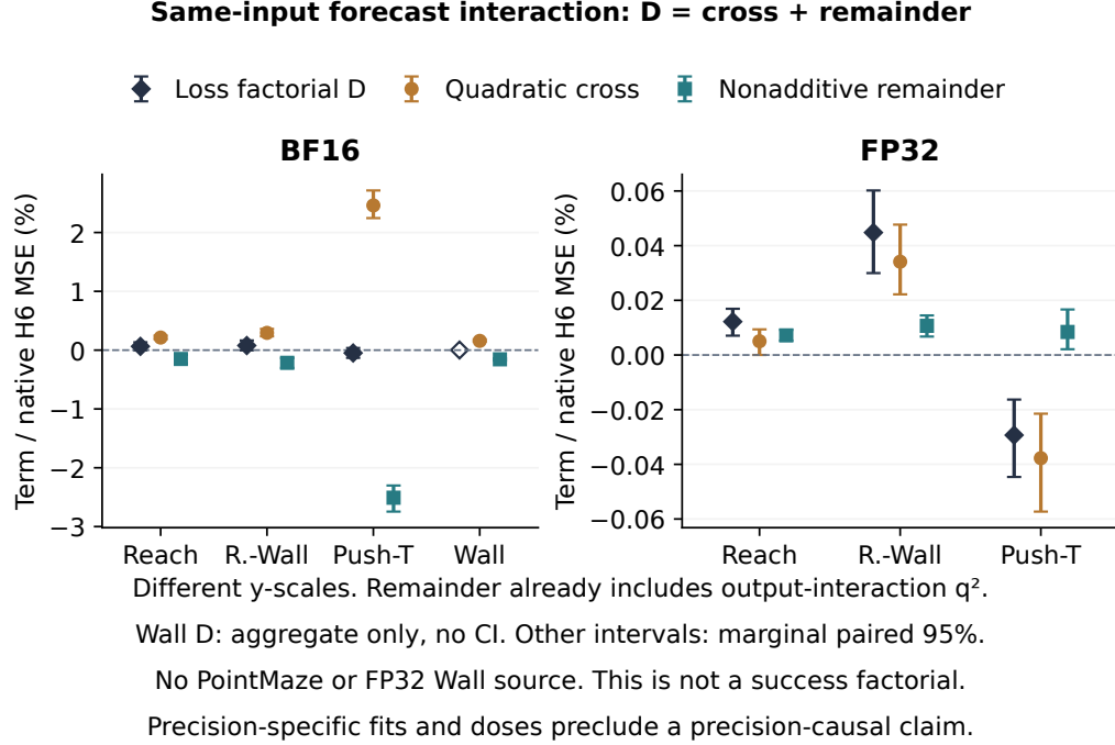
Figure 8: Output pathways and squared-loss interaction are distinct. All seven registered H6 proprioceptive conditions. The additive cross-term plus nonadditive remainder equals the loss factorial; the remainder already includes \|q\|^2 , which is not added twice. Wall’s aggregate-only factorial has no invented interval; its remaining intervals retain the saved fixed native denominator. Separate axis scales, precision-specific fits, and doses preclude treating the panels as a controlled precision experiment. These are fixed-input forecasts, not protected behavioral interactions.
