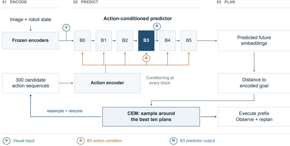
Figure 1: Steering inside a JEPA world model. The predictor forecasts the consequences of candidate action sequences. The planner scores their distance to the encoded goal, refits its action distribution, and repeats. It executes the beginning of the chosen plan before observing and replanning. R marks the four-direction predictor edit; V and A mark the alternative visual and action-conditioning edits. All edits occur at imagined step H3 of an H6 forecast. R is never combined with V/A in the eight-condition evaluation.
