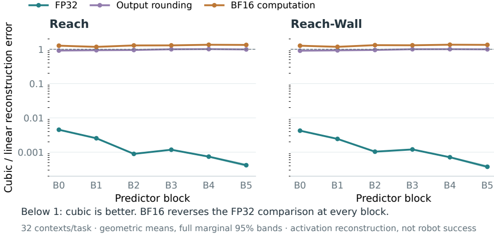
Figure 5: The local reconstruction comparison depends on computation, not only output rounding. Same weights, inputs, action perturbations and coefficients; 32 contexts per task, all six blocks. Curves show geometric mean cubic/linear activation-MSE ratios with full marginal 95% bands. The prespecified paired arithmetic contrasts use six-layer correction. These are reconstruction errors, not forecast or robot-success gains.
