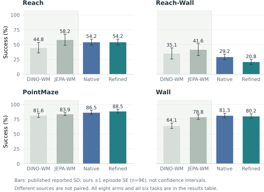
Figure 6: Protected behavior and published benchmarks are distinct evidence. The fixed refined arm and its concurrent native reference use 96 fresh scenarios per task. Shaded DINO-WM/JEPA-WM recipe values are external context. Published error bars are reported late-epoch SD; local bars are one Bernoulli episode SE, not confidence intervals or training-seed variation. No best arm is selected by task. All eight arms and historical rates remain in Appendix C.
