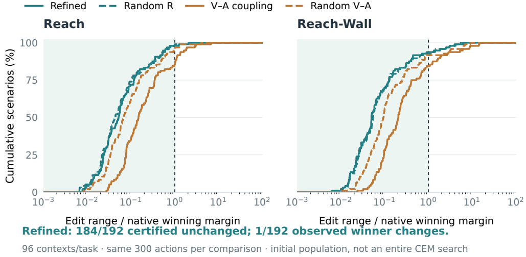
Figure 3: Cost perturbations can be compared with a selection boundary. Complete 192-scenario development diagnostic, one shared 300-candidate bank per scenario. The certificate concerns the initial bank’s winner, not the full iterative CEM solution, later replanning calls, or protected behavior.
