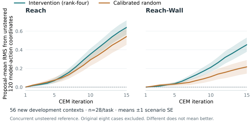
Figure 4: Adaptive search can diverge despite nearly shared initial elites. Complete 56-context extension, both edit arms and all fifteen iterations. Shading is one scenario standard error, not a confidence interval. RMS uses all 120 proposal-mean coordinates; the returned prefix uses 60 coordinates. Entropy curves and every paired returned-prefix endpoint are retained in the public CEM report. This is a search measurement, not a physical-quality test.
