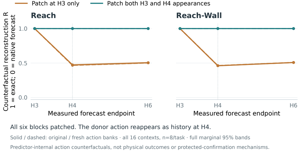
Figure 7: A one-time internal patch is not a coherent action change. The donor H3 condition must also replace the older occurrence at H4. All six blocks, both original/fresh action banks, and all 16 contexts are retained. The exact persistent/raw-action match is a computational consistency control; the H3-only deviation is measured. Bands are full marginal context-bootstrap intervals. No physical actions are executed.
