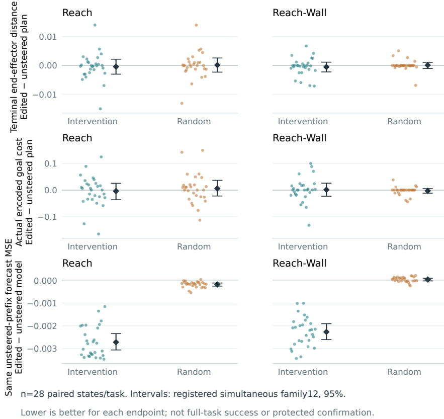
Figure 5: Better forecasts do not establish a better executed prefix. All 56 development states and twelve registered contrasts. Points retain each paired state; diamonds mark means and bars use the prespecified family-twelve 95% intervals. Lower is better for each endpoint. Same-prefix forecast comparisons hold the unsteered-selected actions fixed; physical comparisons execute each edited model’s selected actions. Neither is full-task success.
