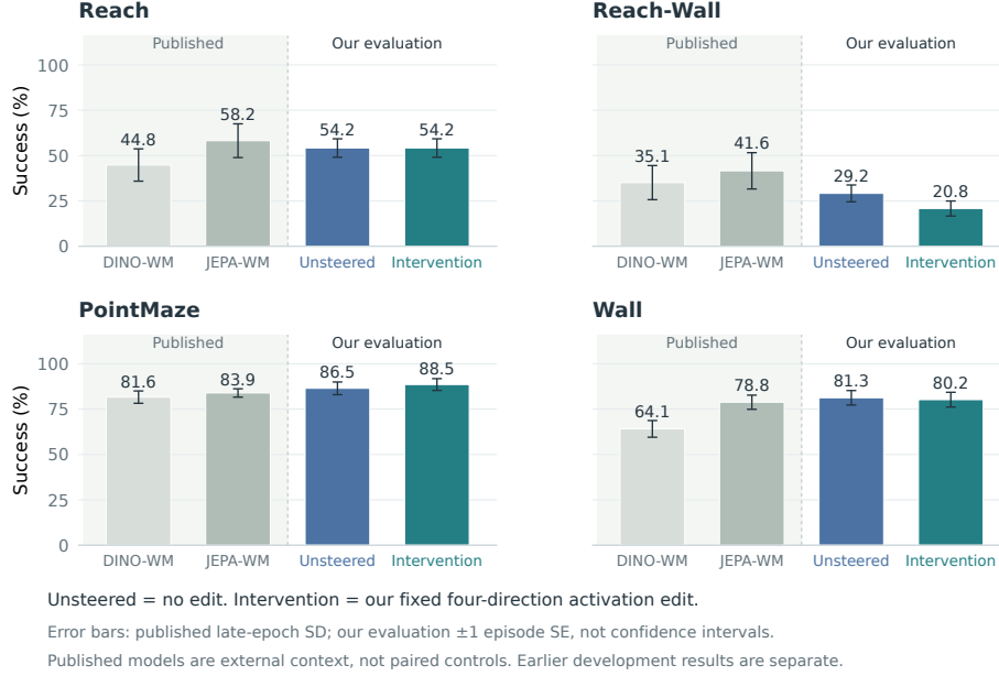
Figure 6: Protected behavior and published benchmarks are distinct evidence. Unsteered denotes the unchanged checkpoint; Intervention denotes the fixed four-direction (rank-four) edit. These paired arms use 96 fresh scenarios per task. Shaded DINO-WM/JEPA-WM recipe values are external context. Published error bars are reported late-epoch SD; local bars are one Bernoulli episode SE, not confidence intervals or training-seed variation. No best arm is selected by task. All eight arms and historical rates remain in Appendix C.
