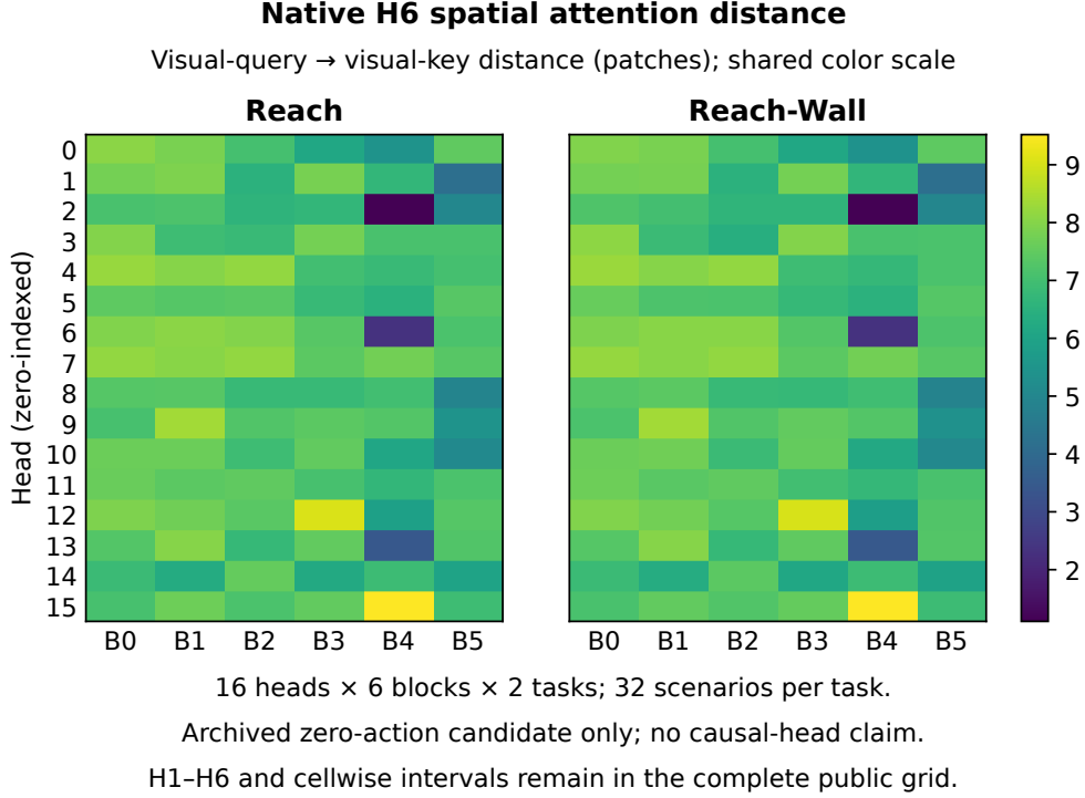
Figure 8: Native H6 attention distance, all six blocks and sixteen heads. Each cell averages 32 development contexts per task with the same archived zero-action candidate. Colors are shared across tasks. The complete H1-H6 grid is retained in the accompanying data. Attention distance is not causal importance or evidence of a planning-emergence zone.
