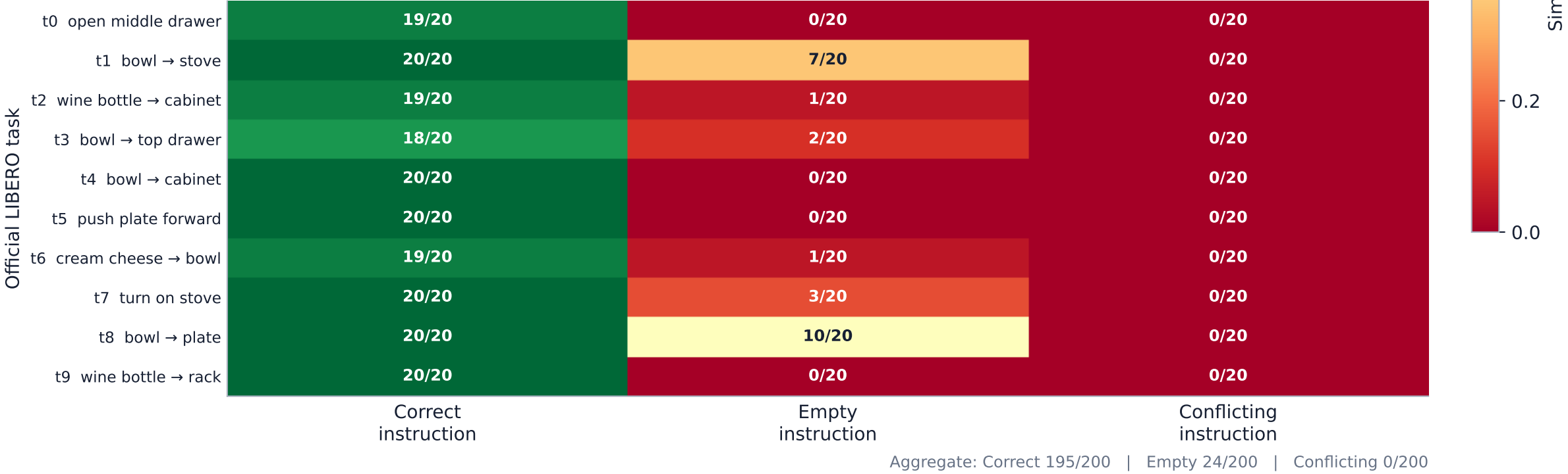
c LIBERO Goal: behavior depends strongly on the instruction
