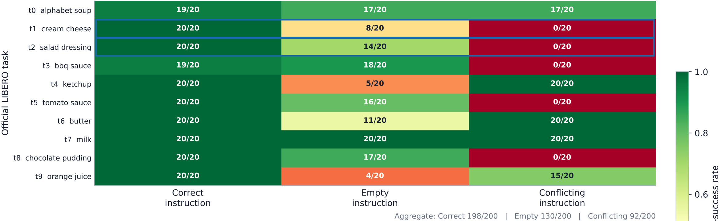
b LIBERO Object: some tasks persist without the right instruction
