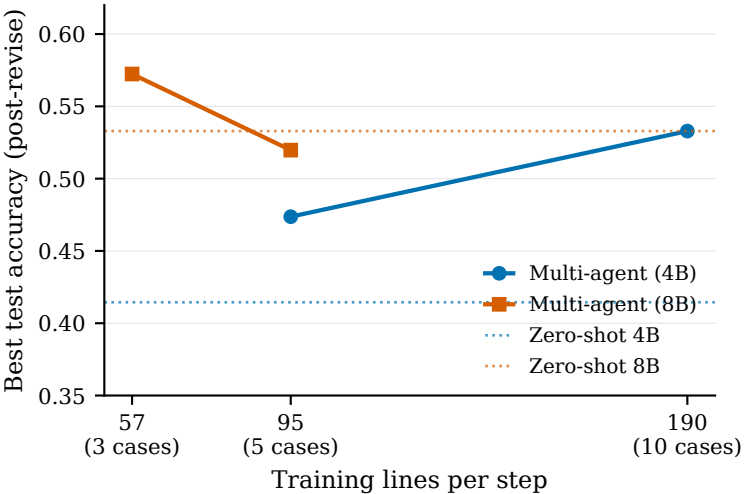
(a) Scaling with training data
