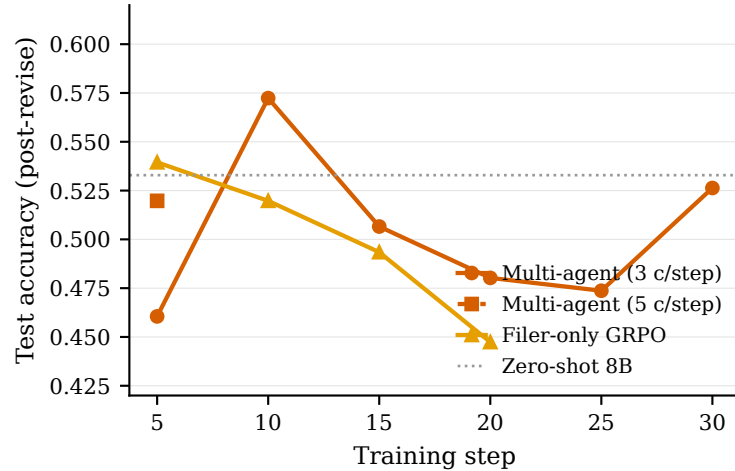
(c) Qwen3-8B training trajectories
