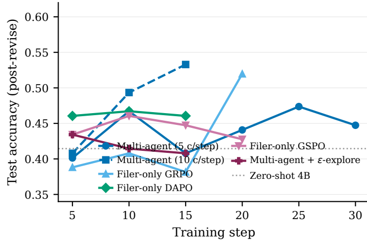
(b) Qwen3-4B training trajectories
