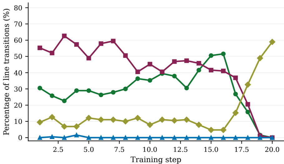
Case-mix dynamics during training (4b_10_v2)
