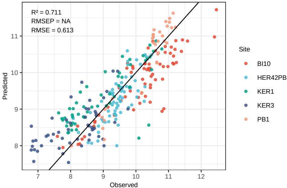
Fe WLS_weighted – Predicted vs Observed
