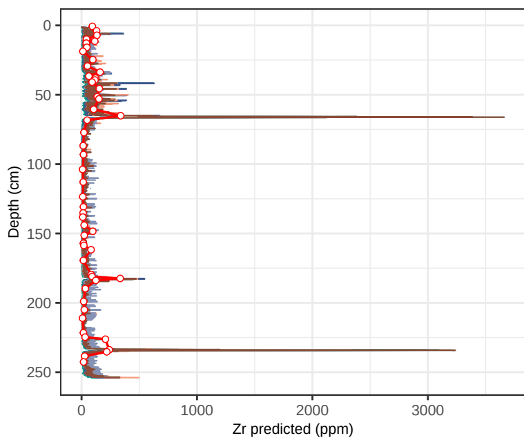
Site KER1 – Zr (depth, all models)
