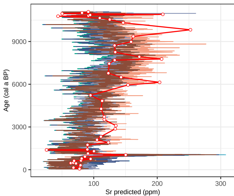
Site KER3 – Sr (age vs ppm, all)
