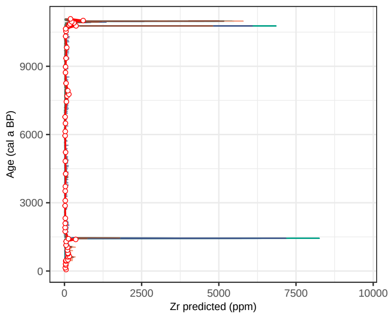
Site KER3 – Zr (age vs ppm, all)
