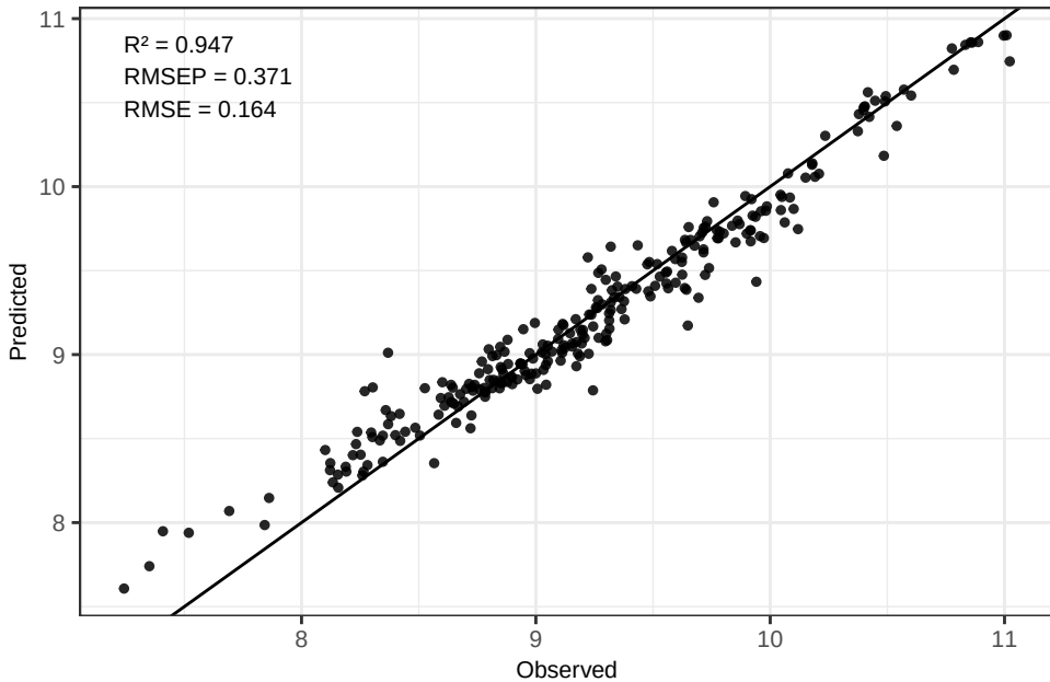
Ca – RF Predicted vs Observed (log-space)
