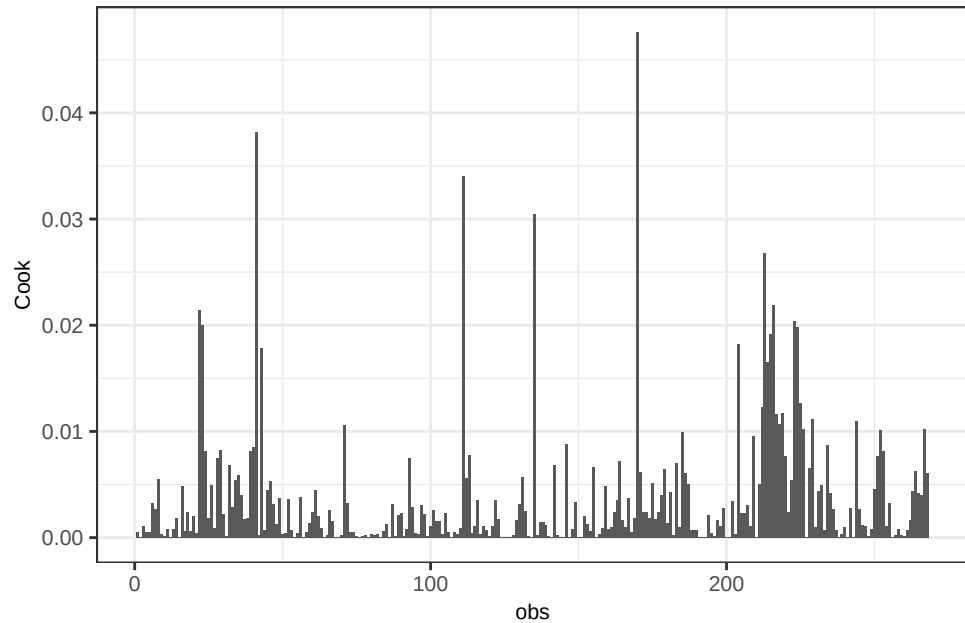
Fe OLS – Cook's Distance
