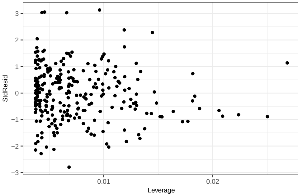
Fe OLS – Leverage Plot
