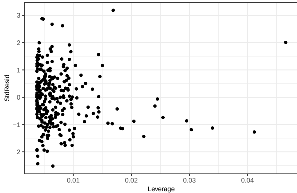
Fe WLS - Leverage Plot
