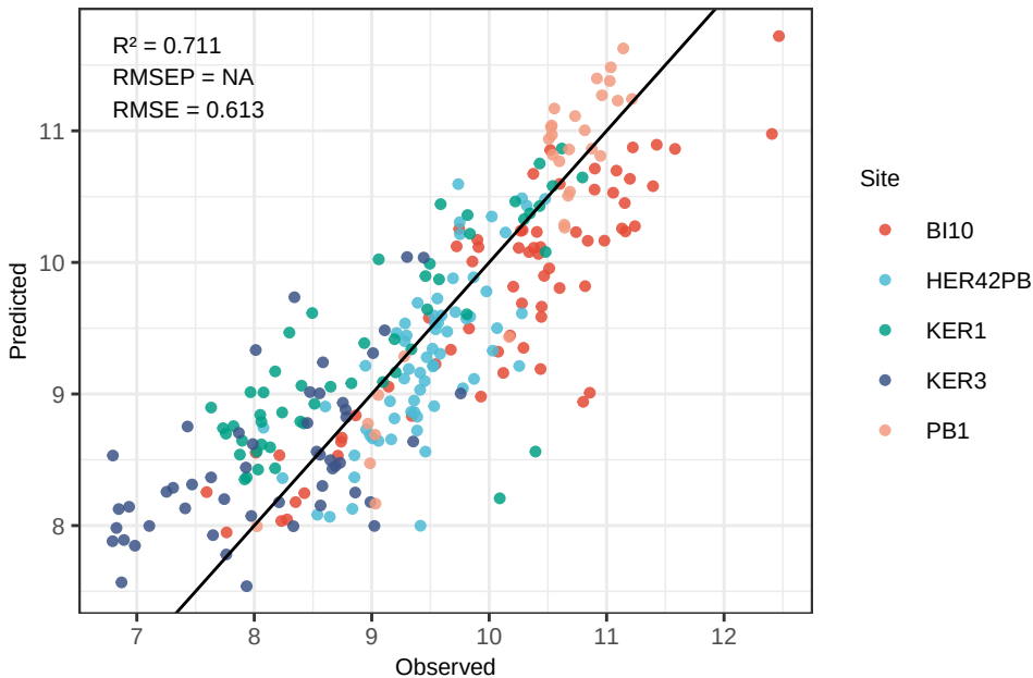
Fe WLS_weighted - Predicted vs Observed (log-space)
