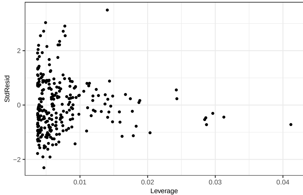
Mn – OLS Leverage vs Std. Residual
