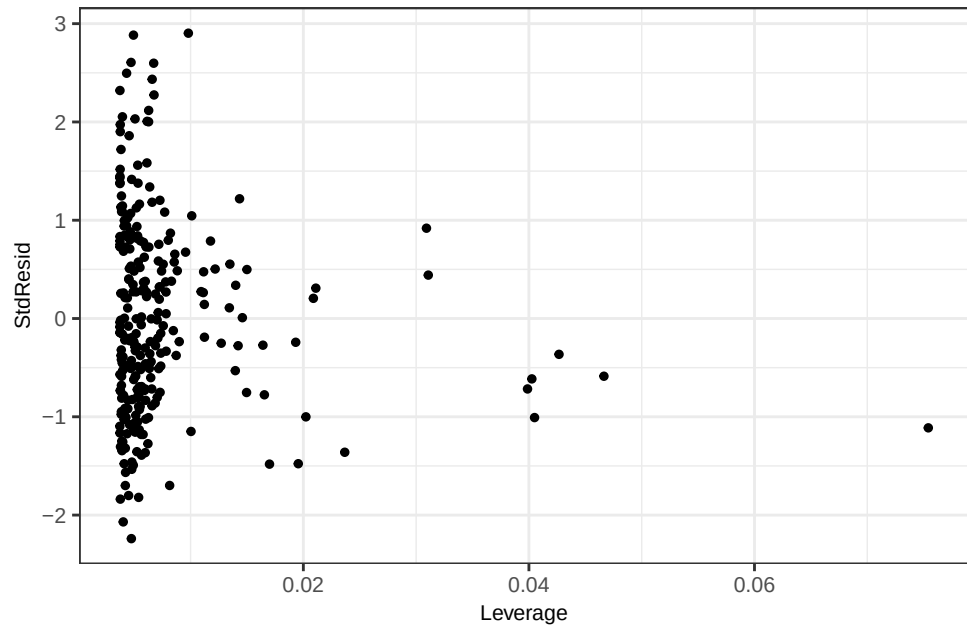
Mn - WLS(wt) Leverage vs Std. Residual
