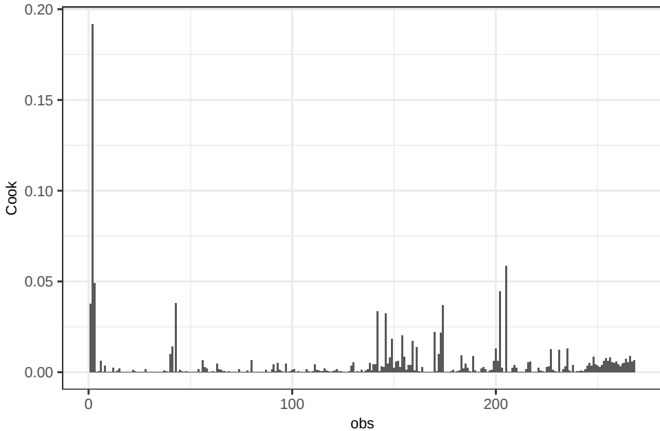
Sr - WLS(wt) Cook's distance
