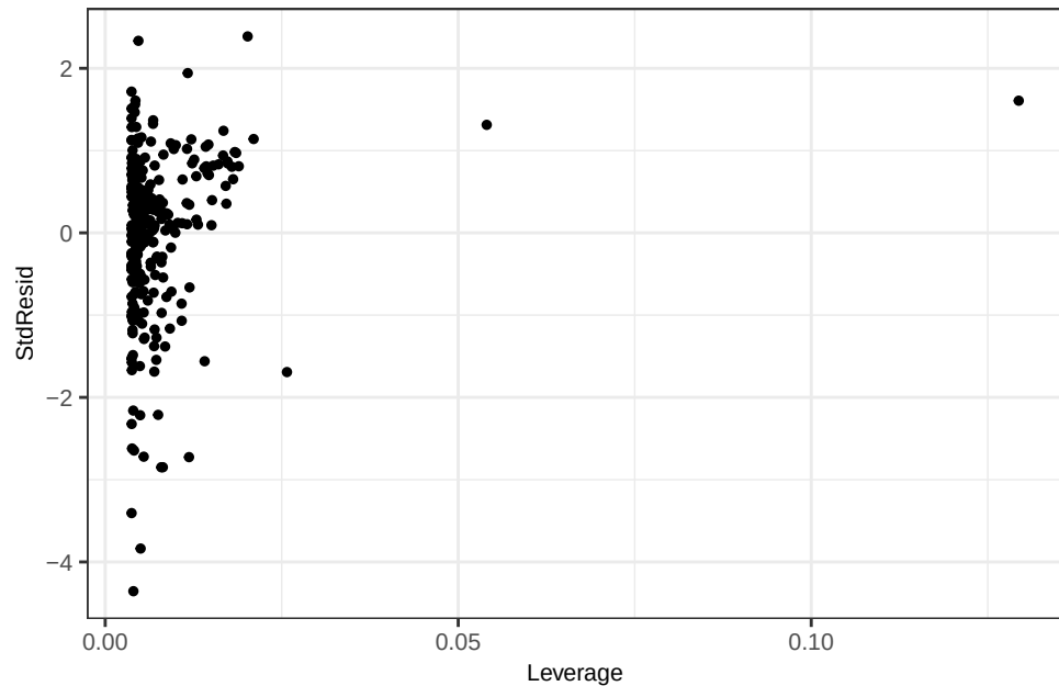
Sr – WLS(wt) Leverage vs Std. Residual
