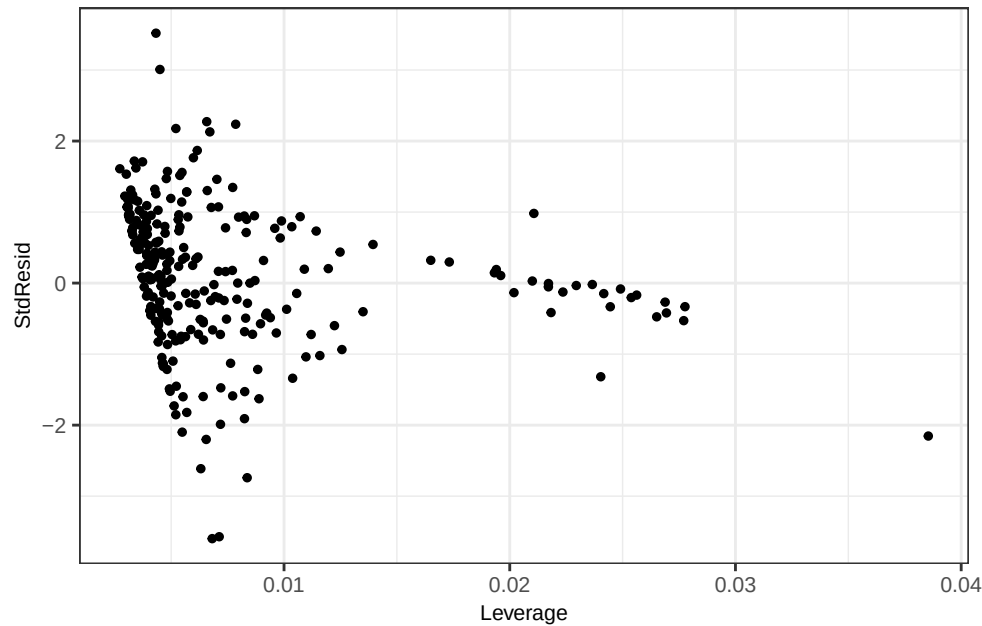
Ti - OLS(wt) Leverage vs Std. Residual
