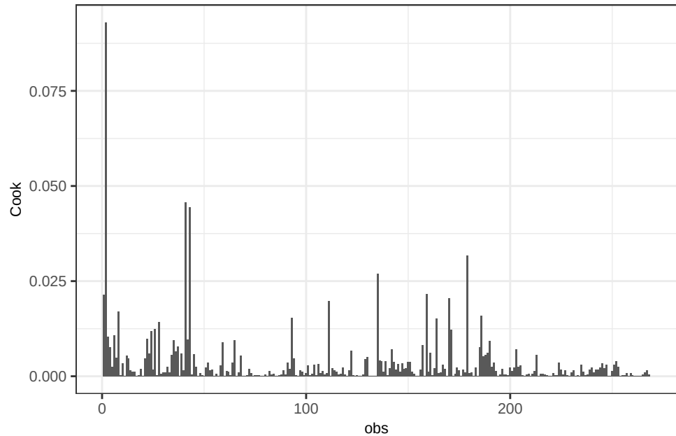
Ti - OLS(wt) Cook's distance
