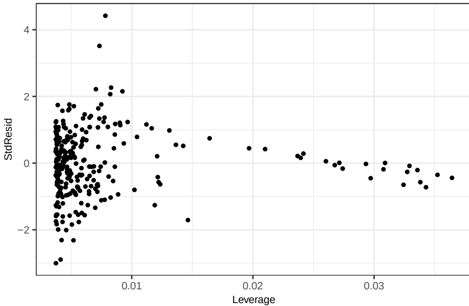
Ti – OLS Leverage vs Std. Residual
