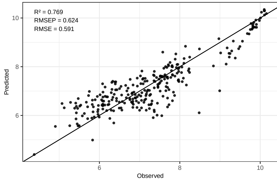
Ti – Bayes Predicted vs Observed (log-space)
