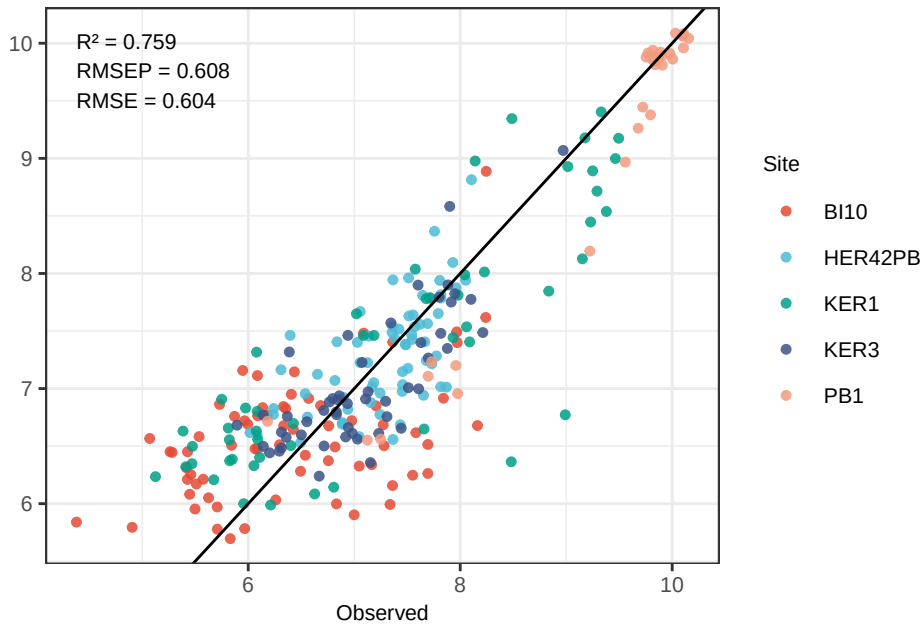
Ti RF – Predicted vs Observed (log-space)
