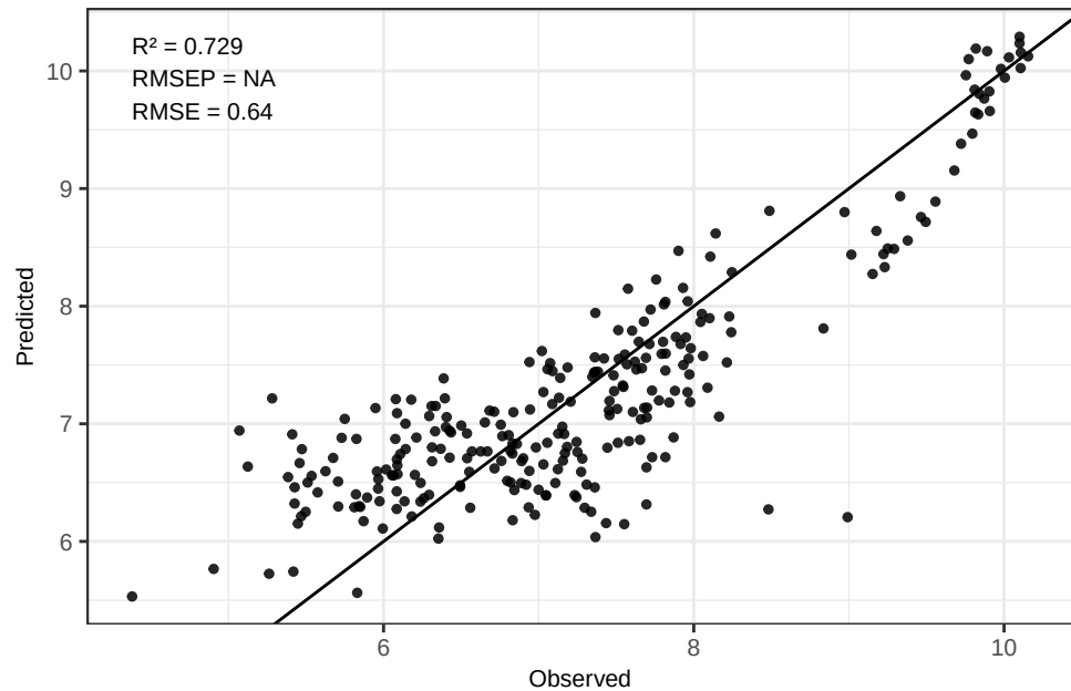
Ti - WLS(wt) Predicted vs Observed (log-space)
