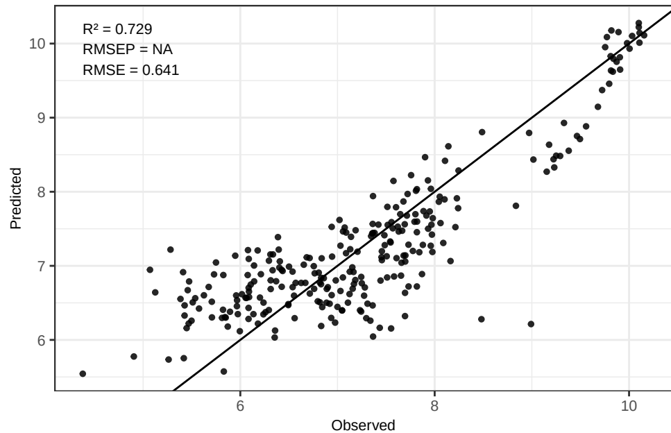
Ti - WLS Predicted vs Observed (log-space)
