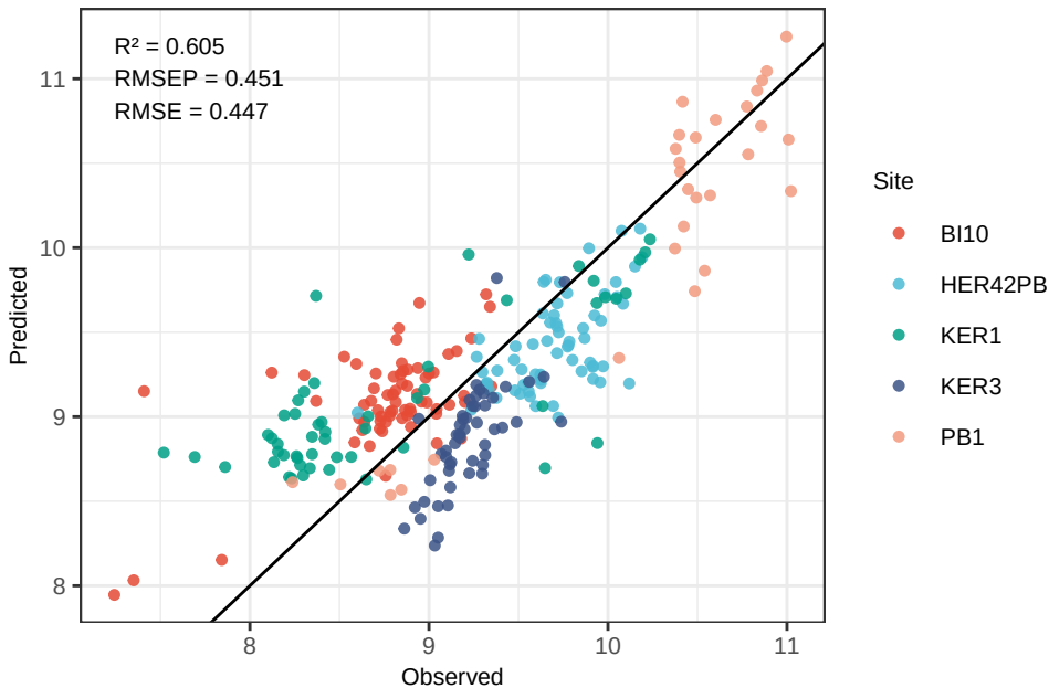
Ca OLS – Predicted vs Observed (log-space)
