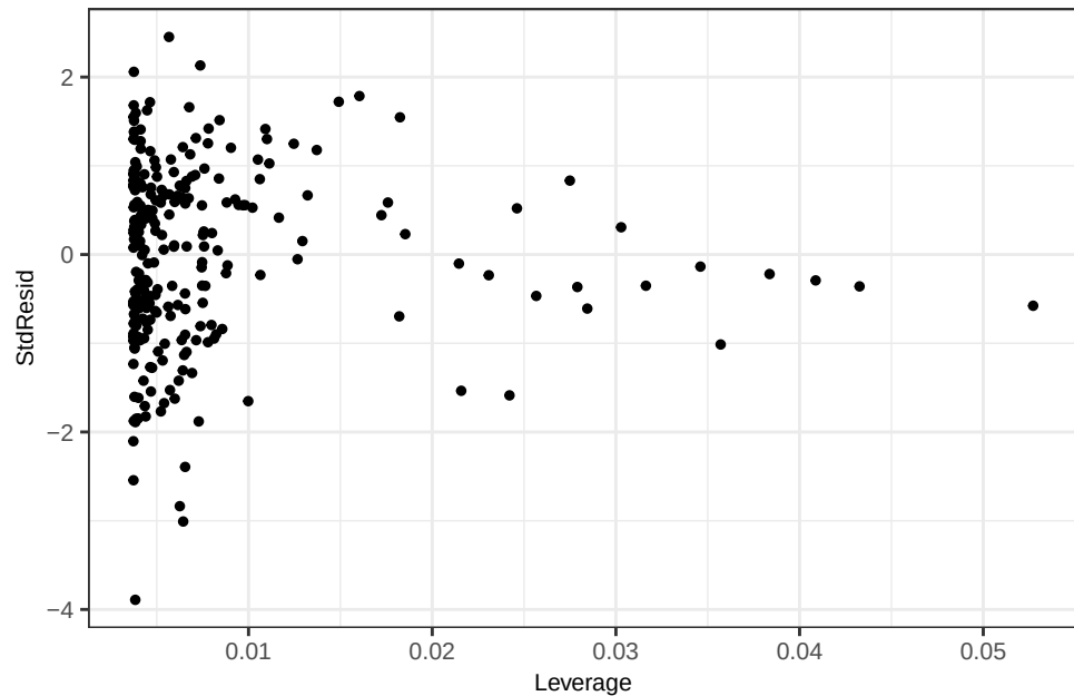
Ca – OLS Leverage vs Std. Residual
