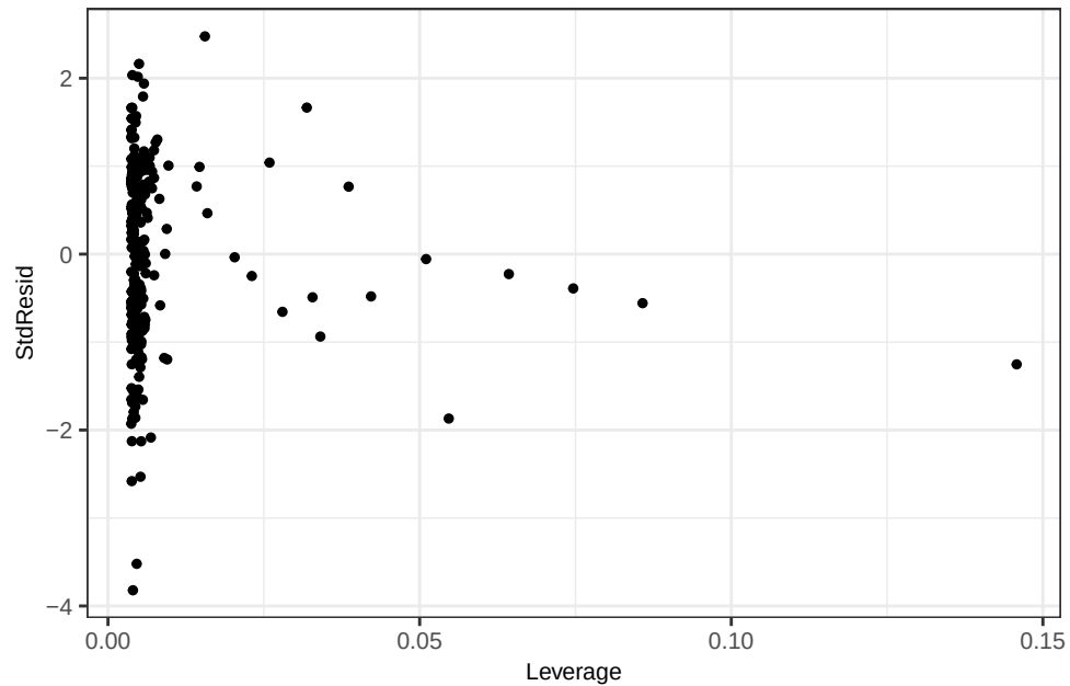
Ca - WLS(wt) Leverage vs Std. Residual
