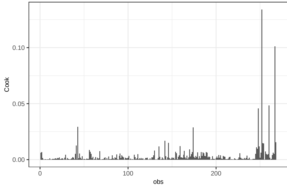
Ca - WLS(wt) Cook's distance
