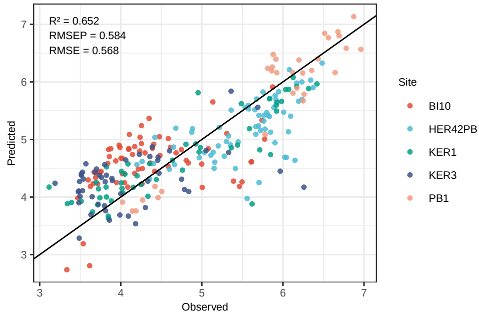
Mn PLS_kfold - Predicted vs Observed (log-space)
