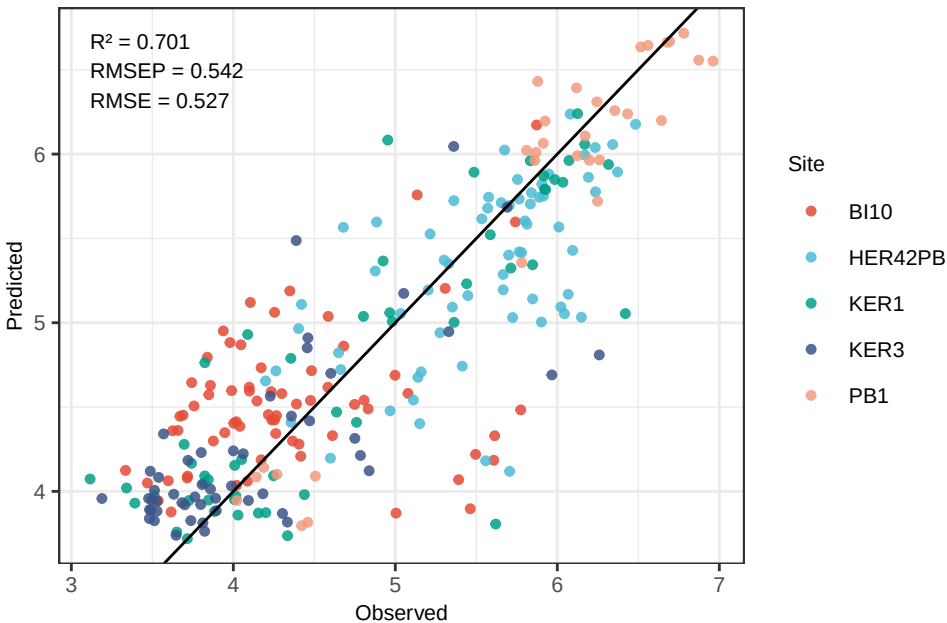
Mn RF – Predicted vs Observed (log-space)
