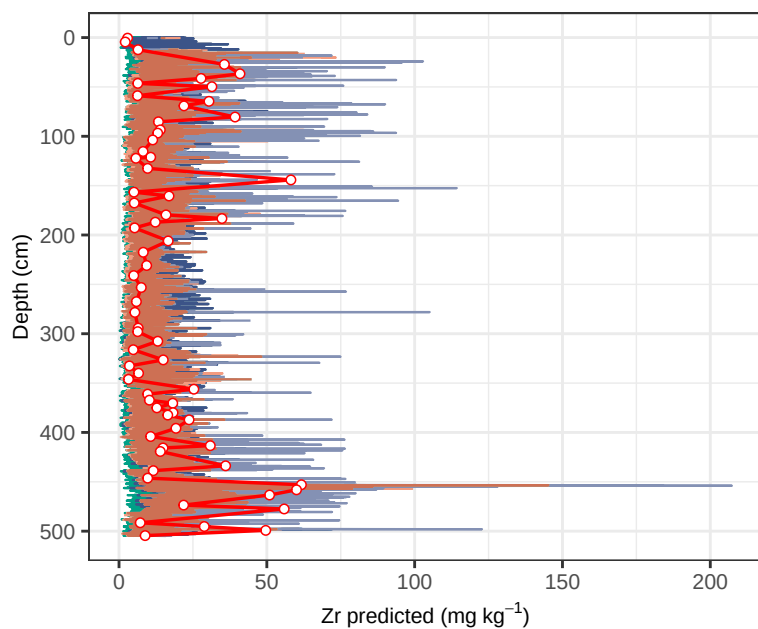
Site BI10 – Zr (depth, all models)
