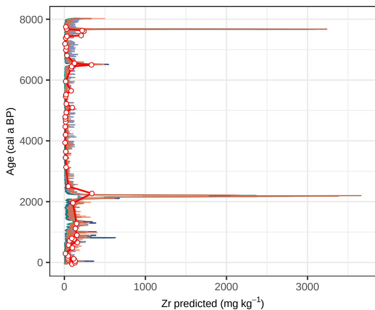
Site KER1 – Zr (age vs mg kg -1 , all)
