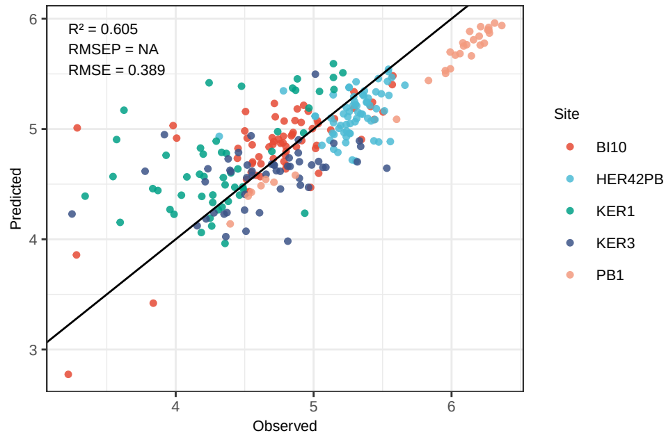
Sr WLS_weighted – Predicted vs Observed (log-space)
