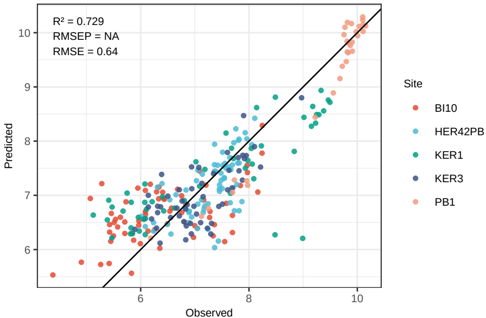
Ti WLS_weighted – Predicted vs Observed (log-space)
