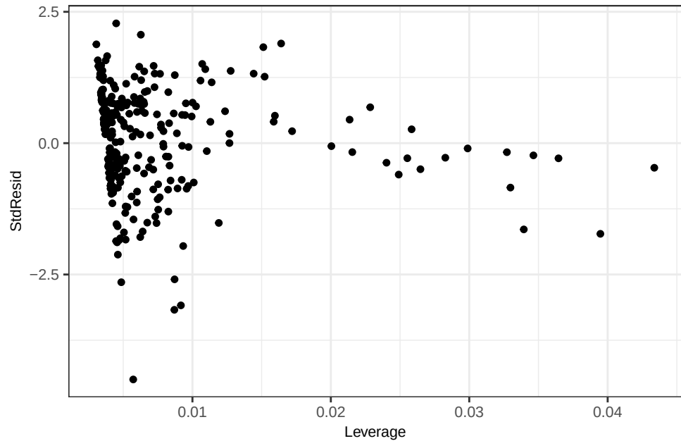
Ca OLS_weighted – Leverage
