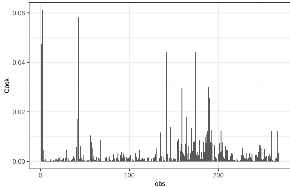
Ca OLS_weighted – Cook's Distance
