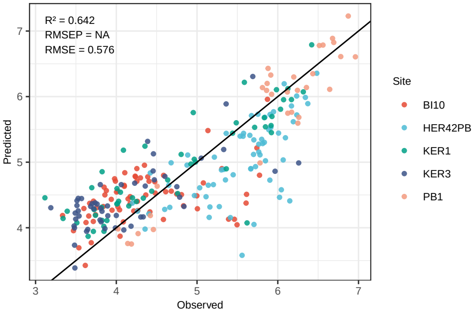
Mn WLS_weighted – Predicted vs Observed
