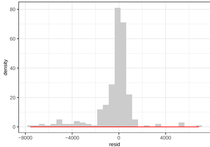
Ti Bayes – ACE Residuals
