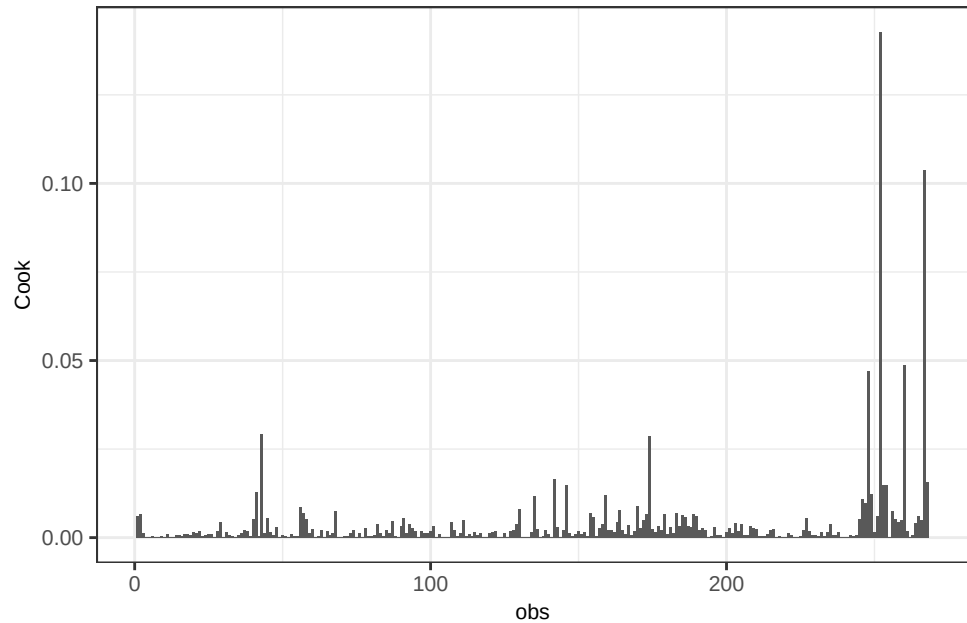
Ca WLS - Cook's Distance
