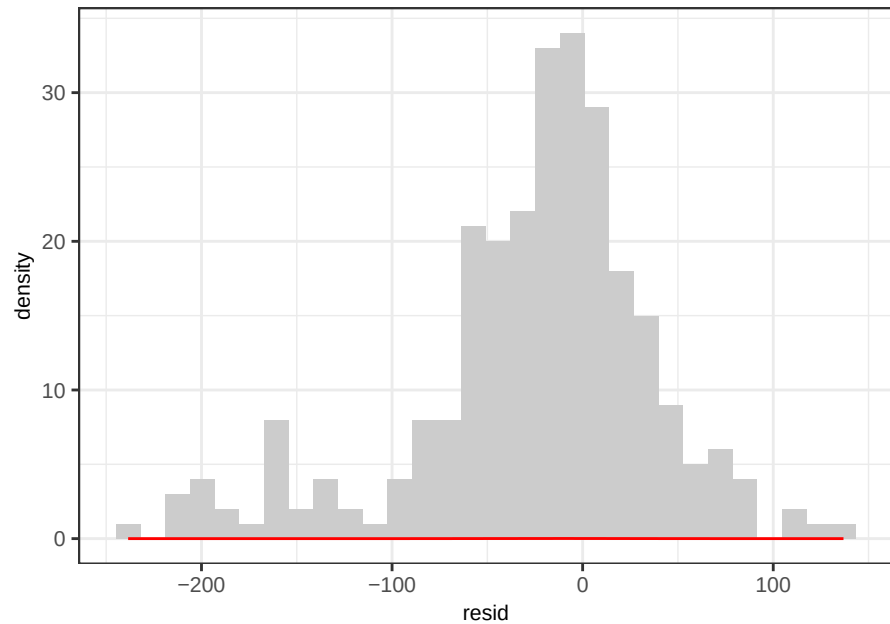
Sr OLS_weighted - ACE Residuals
