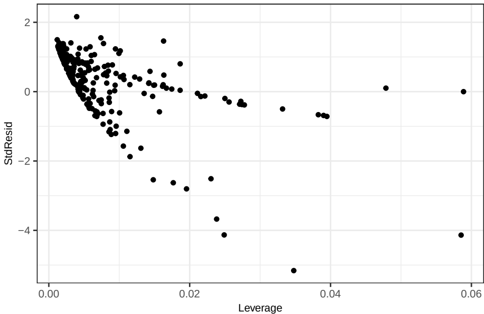
Zr OLS_weighted - Leverage
