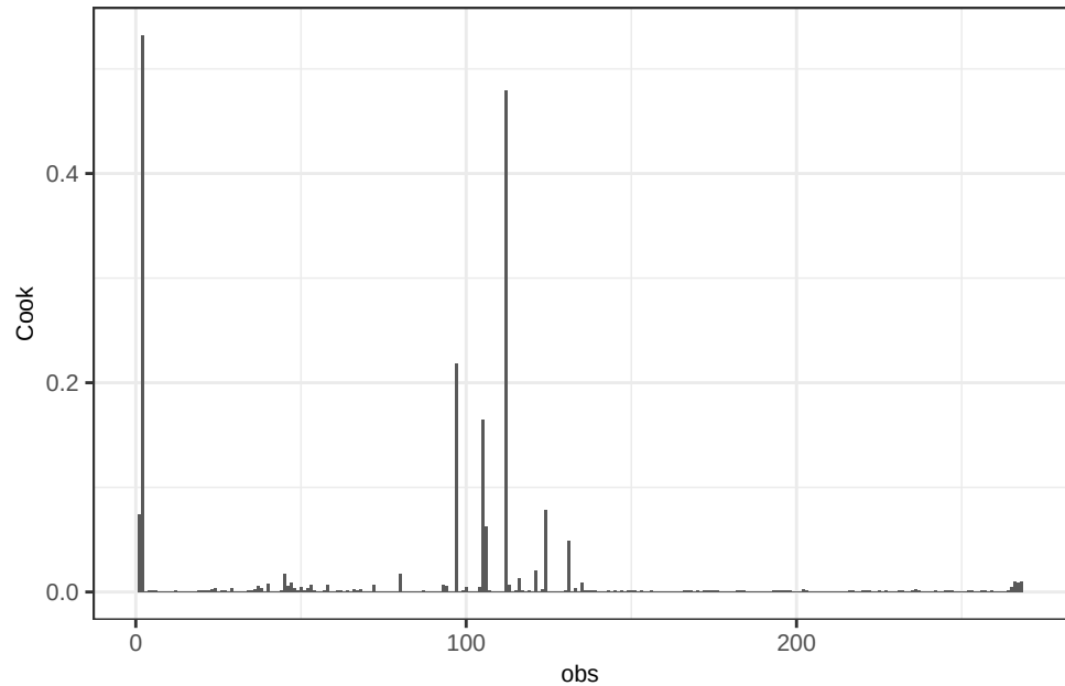
Zr OLS_weighted – Cook's Distance
