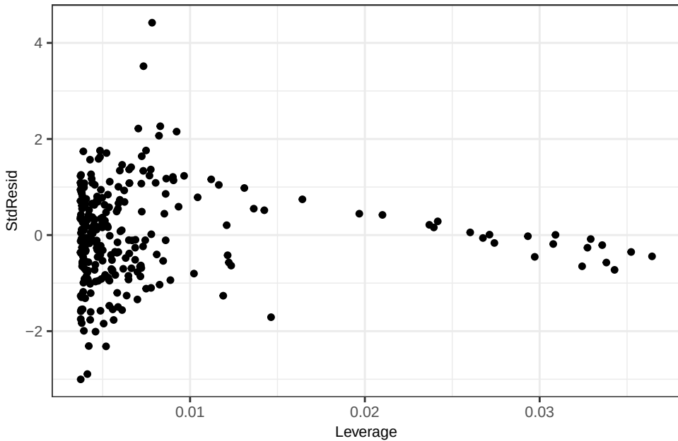
Ti OLS - Leverage
