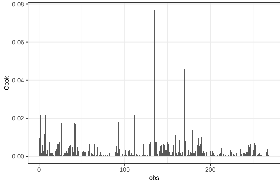
Ti OLS – Cook's Distance
